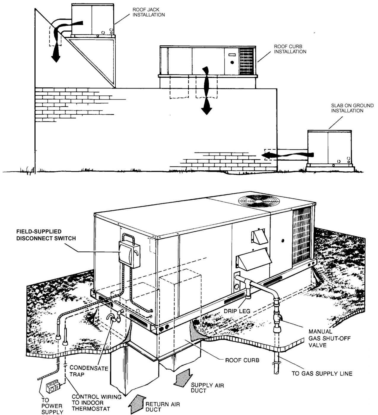
FIGURE 9 - TYPICAL APPLICATIONS
