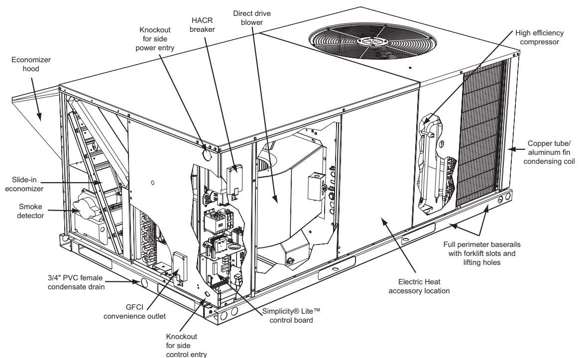
FIGURE 1 - UNIT CUTAWAY
